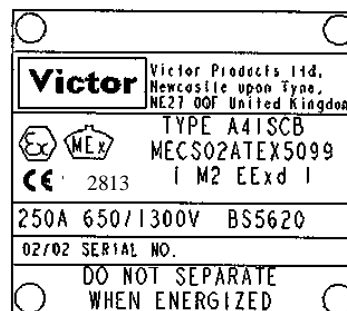
NAMEPLATE DETAIL BOLTED COUPLER
