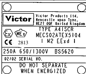
NAMEPLATE DETAIL RESTRAINED COUPLER
