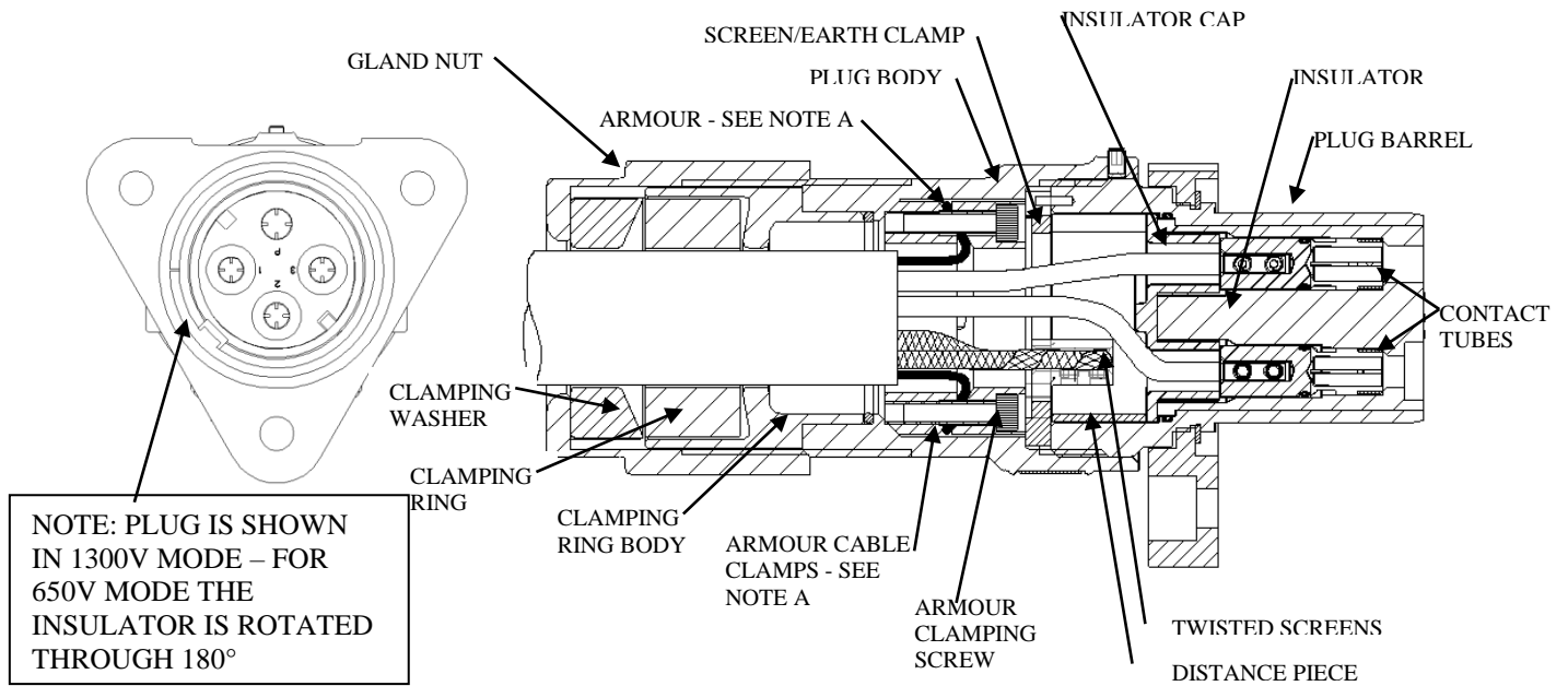
Fig.1 BOLTED PLUG FOR SCREENED AND/OR P.W.A. CABLE
