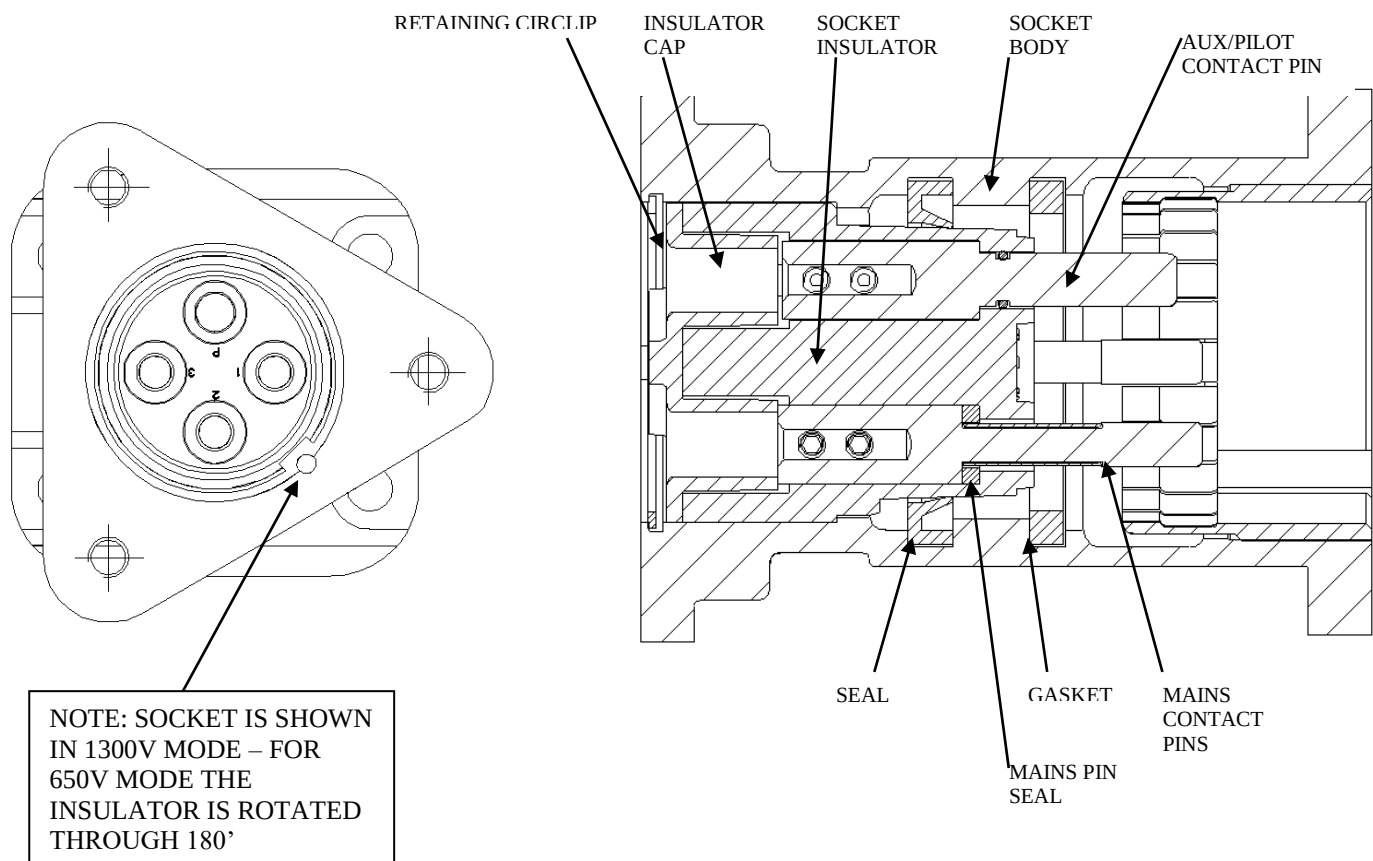
Fig.1 BOLTED SOCKET
