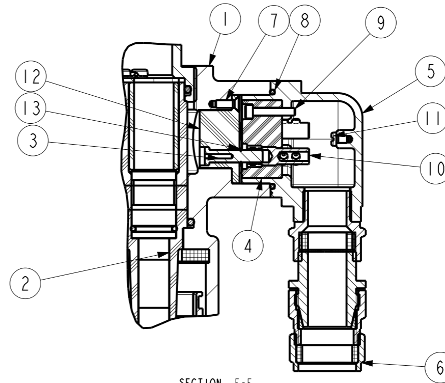
SECTION E-E
